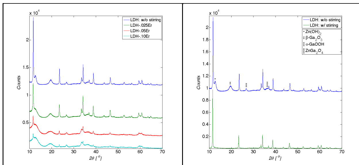
(a) (b) Figure 5.1 XRD data for (a) all LDH samples and (b) LDH with and without stirring.
